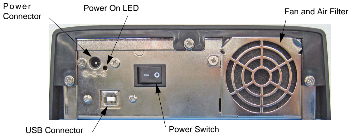
Figure 1. UDO60D-u Back View
