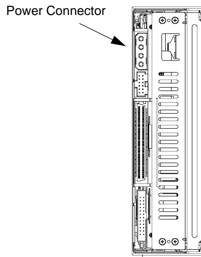
Figure 9. Proper Vertical Orientation for UDO60I
