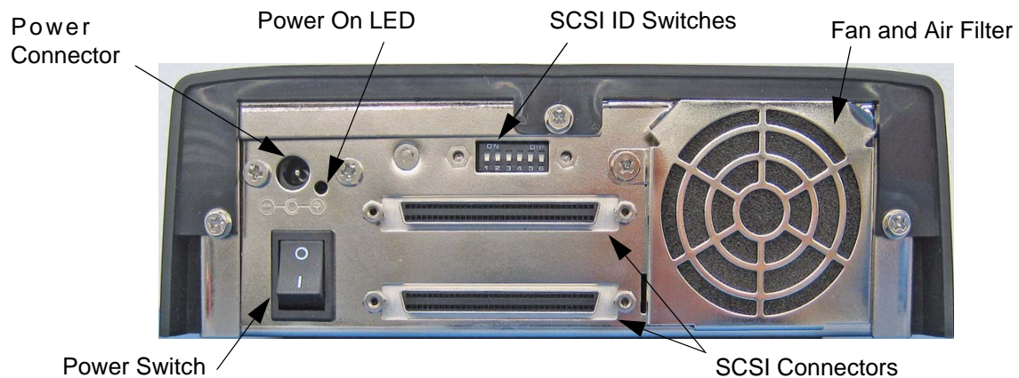
Figure 2. UDO60D-s Back View
