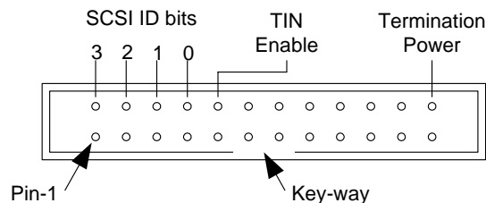
Figure 10. UDO60I Function Connector Jumper Options
