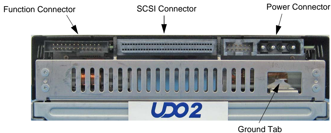
Figure 5. UDO60I-s Back View
